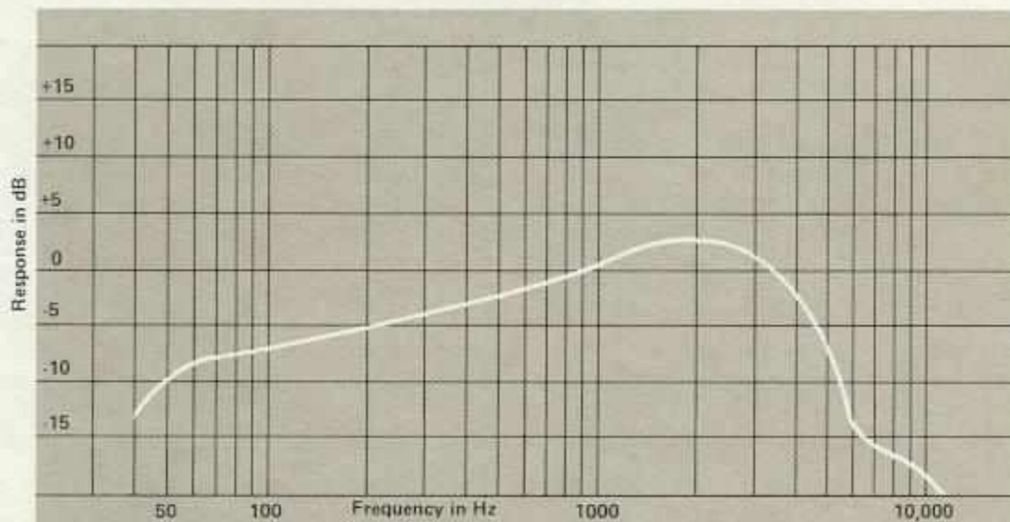
Frequency response contour of Model 2135. Measured response of a typical production unit, including all peaks and dips, does not deviate more than 3 dB from the above curve.
